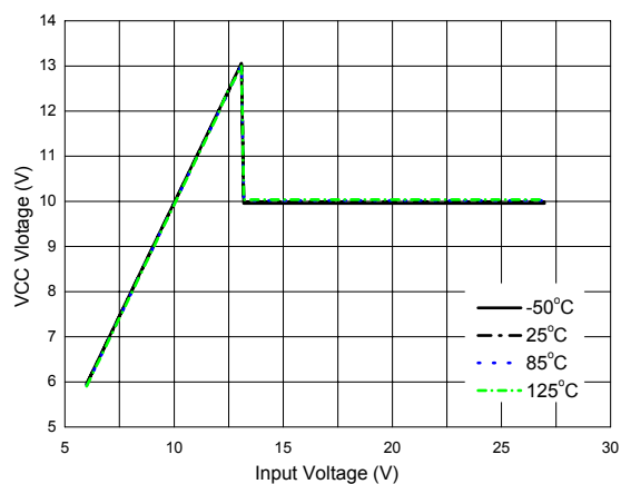
Figure 9. VCC Voltage vs. Input Voltage
