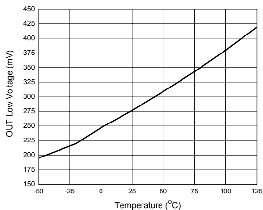
Figure 18. OUT Low Voltage vs. Case Temperature
