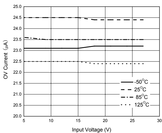
Figure 16. OV Current vs. Input Voltage
