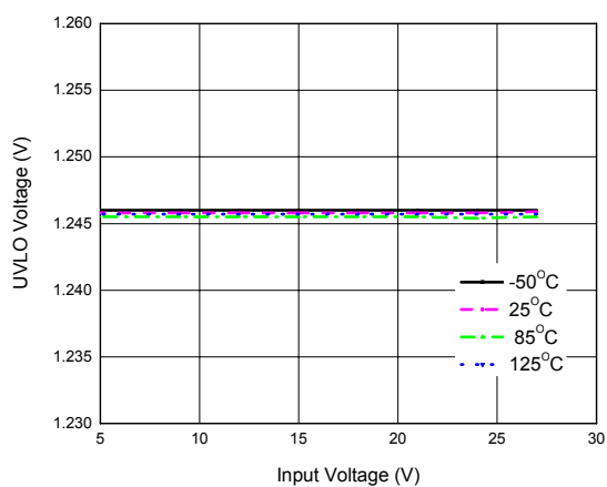
Figure 13. UVLO Voltage vs. Input Voltage
