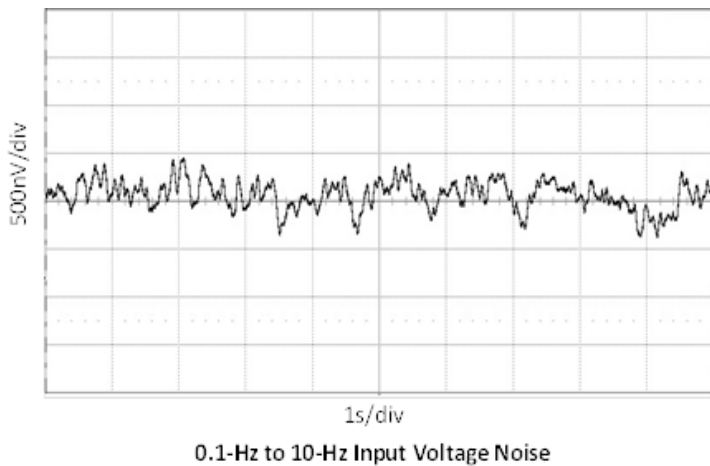
0.1-Hz to 10-Hz Input Voltage Noise
