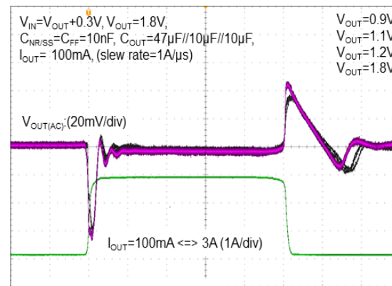
Load transient response vs. V_{OUT}
