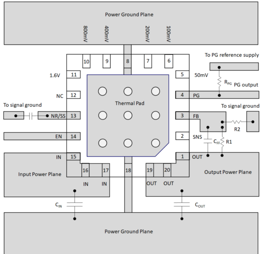
Figure 6. PCB Layout Guide
