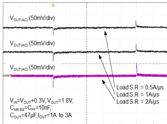
Load transient response vs. load slew rate
