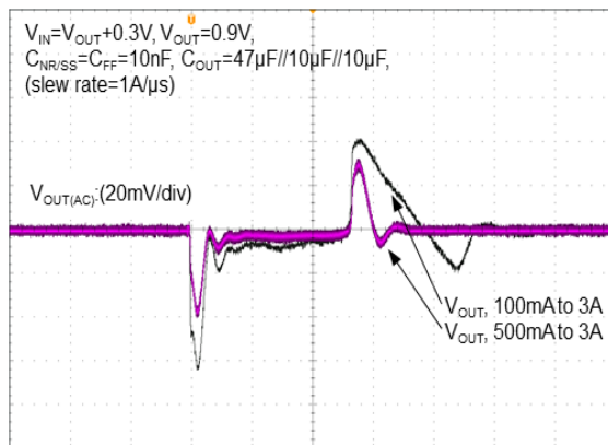
Load transient response vs. DC load
