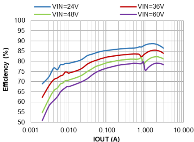
Figure 9. PFM Efficiency vs. IOUT, VOUT=3.3V, L=5.5μH
