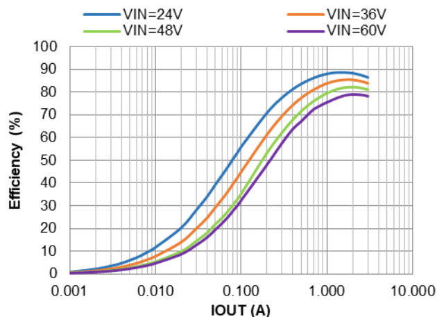
Figure 10. PWM Efficiency vs. IOUT, VOUT=3.3V, L=5.5μH
