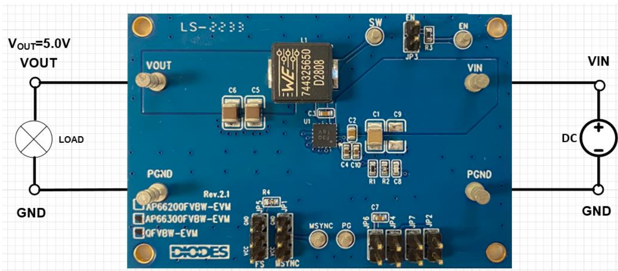
Figure 1. AP66300QFVBW-EVM
