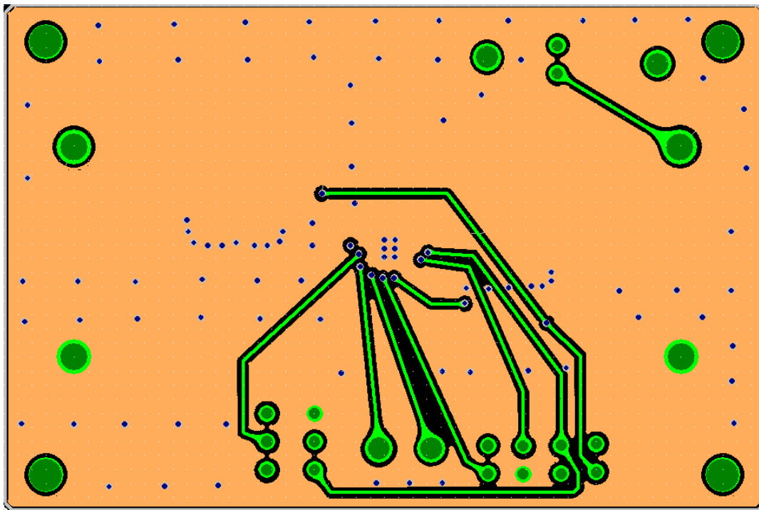
Figure 5. AP66300QFVBW-EVM – Layer 3
