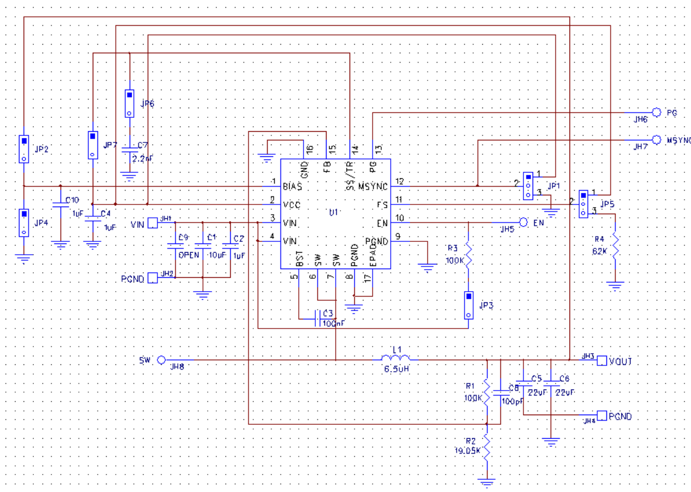
Figure 2. AP66300QFVBW-EVM Schematic
