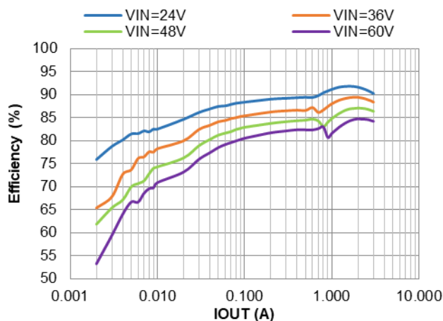
Figure 7. PFM Efficiency vs. IOUT, VOUT=5V, L=6.5μH
