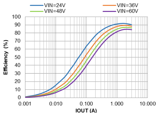
Figure 8. PWM Efficiency vs. IOUT, VOUT=5V, L=6.5μH
