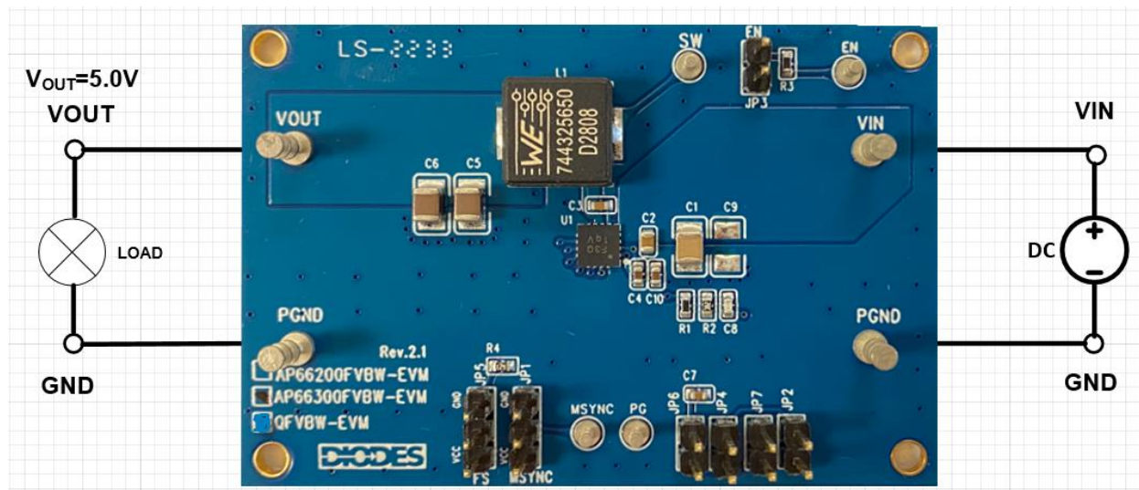
Figure 1. AP66300FVBW-EVM
