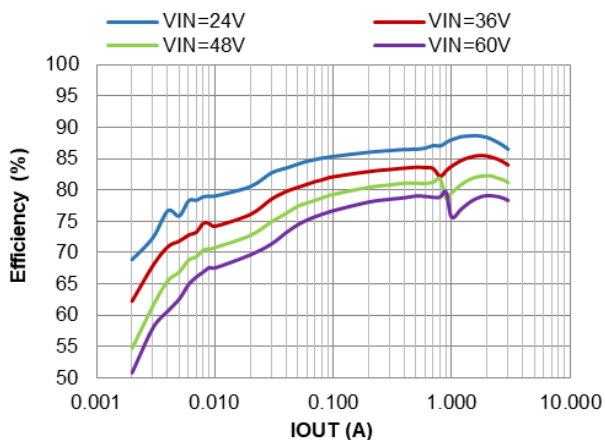
Figure 9. PFM Efficiency vs. IOUT, VOUT=3.3V, L=5.5μH
