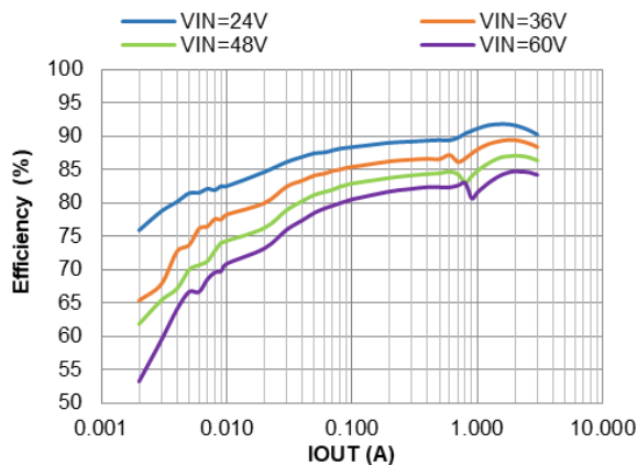
Figure 7. PFM Efficiency vs. IOUT, VOUT=5V, L=6.5μH
