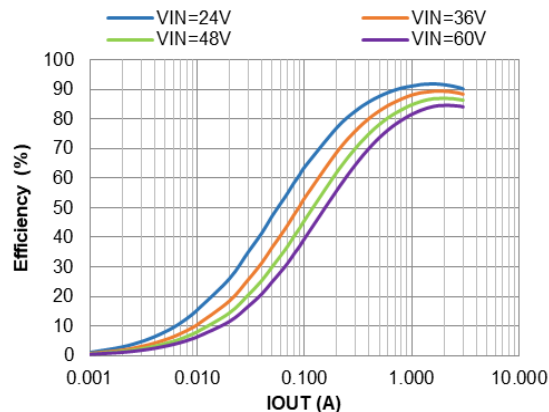
Figure 8. PWM Efficiency vs. IOUT, VOUT=5V, L=6.5μH
