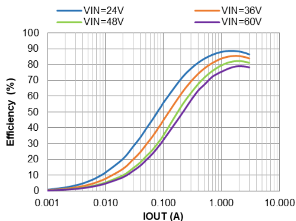
Figure 10. PWM Efficiency vs. IOUT, VOUT=3.3V, L=5.5μH
