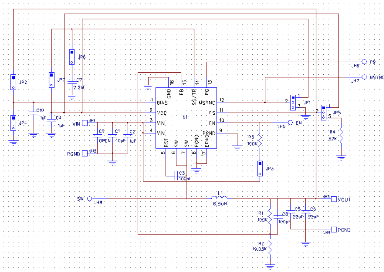
Figure 2. AP66300FVBW-EVM Schematic
