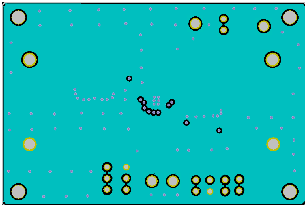
Figure 4. AP66300FVBW-EVM – Layer 2
