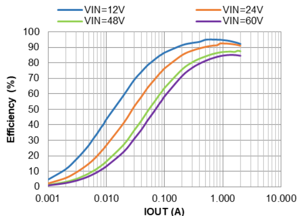
Figure 8. PWM Efficiency vs. IOUT, VOUT=5V, L=10μH
