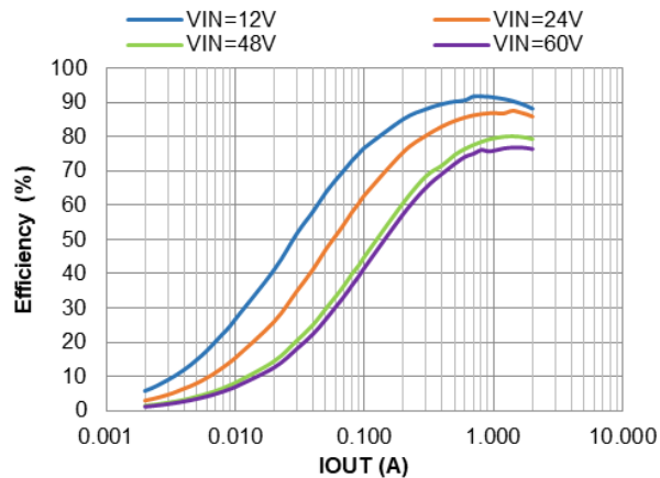
Figure 10. PWM Efficiency vs. IOUT, VOUT=3.3V, L=8.2μH
