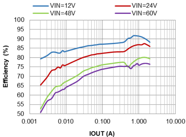
Figure 9. PFM Efficiency vs. IOUT, VOUT=3.3V, L=8.2μH
