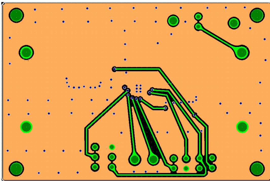
Figure 5. AP66200QFVBW-EVM – Layer 3
