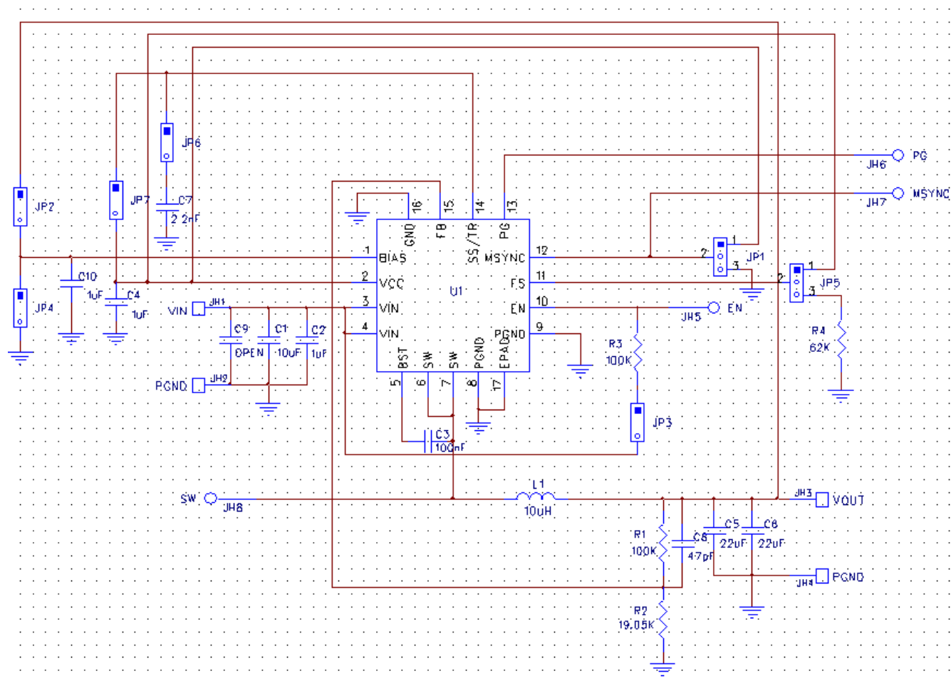
Figure 2. AP66200QFVBW-EVM Schematic
