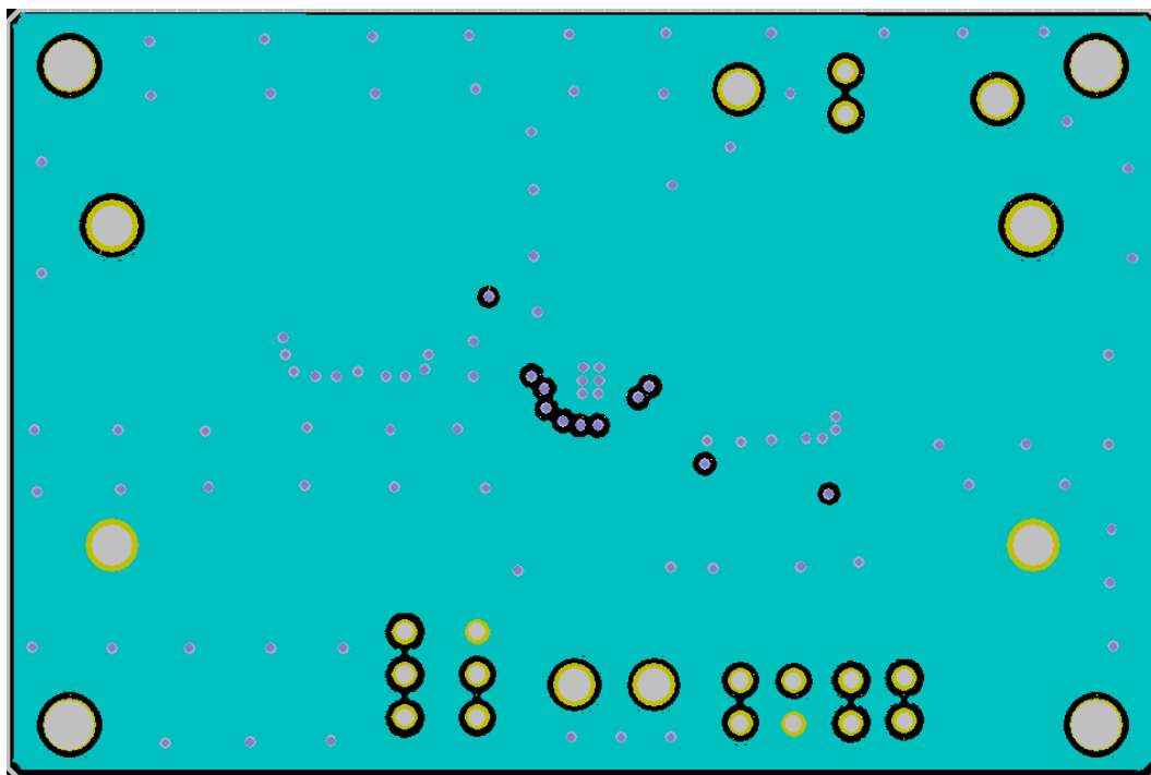
Figure 4. AP66200QFVBW-EVM – Layer 2
