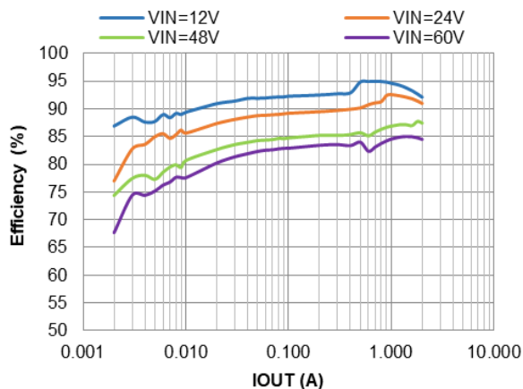
Figure 7. PFM Efficiency vs. IOUT, VOUT=5V, L=10μH
