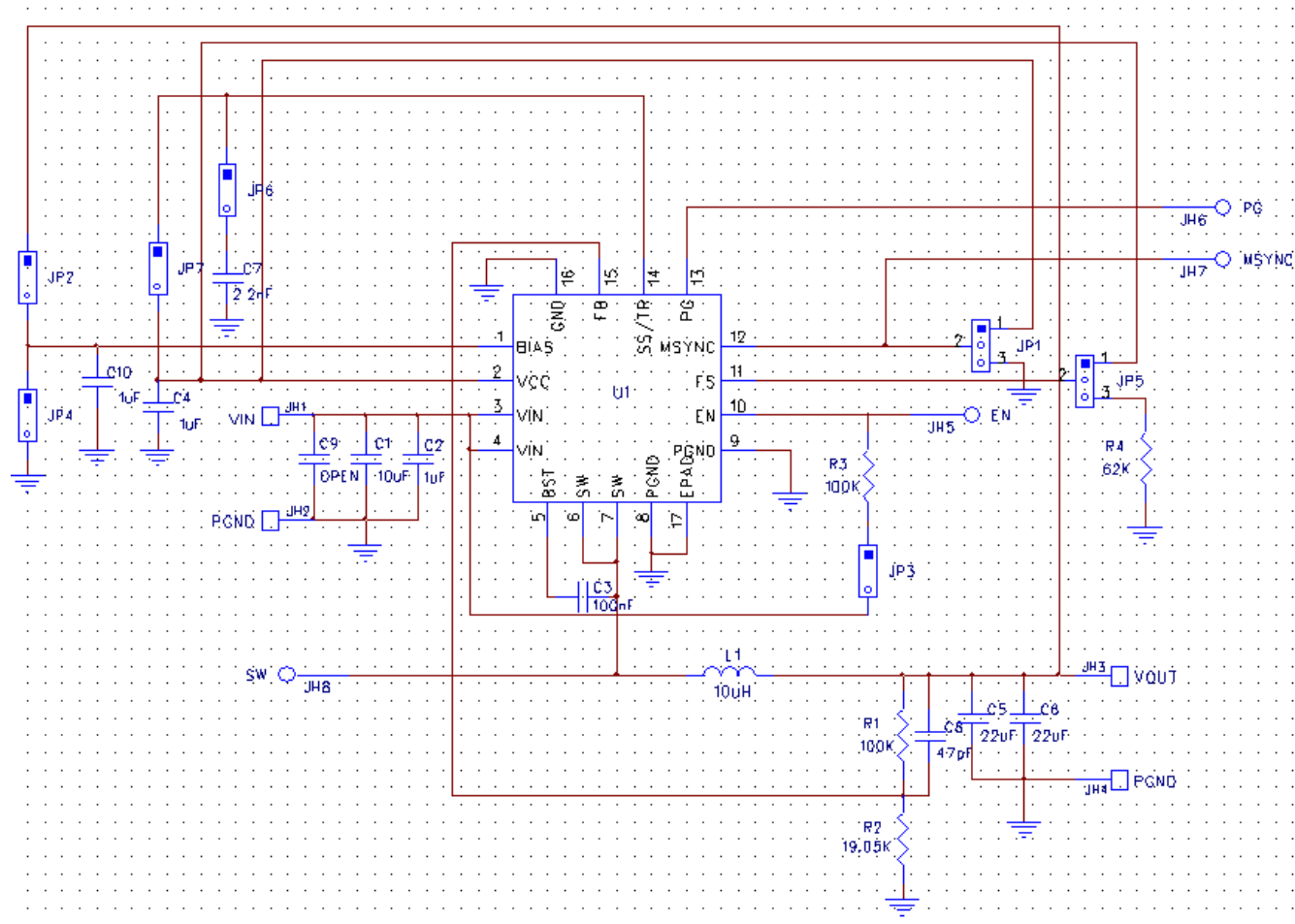
Figure 3. AP66200FVBW-EVM Schematic
