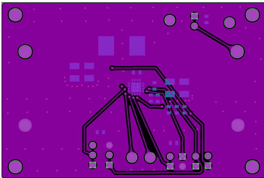
Figure 6. AP66200FVBW-EVM – Layer 3
