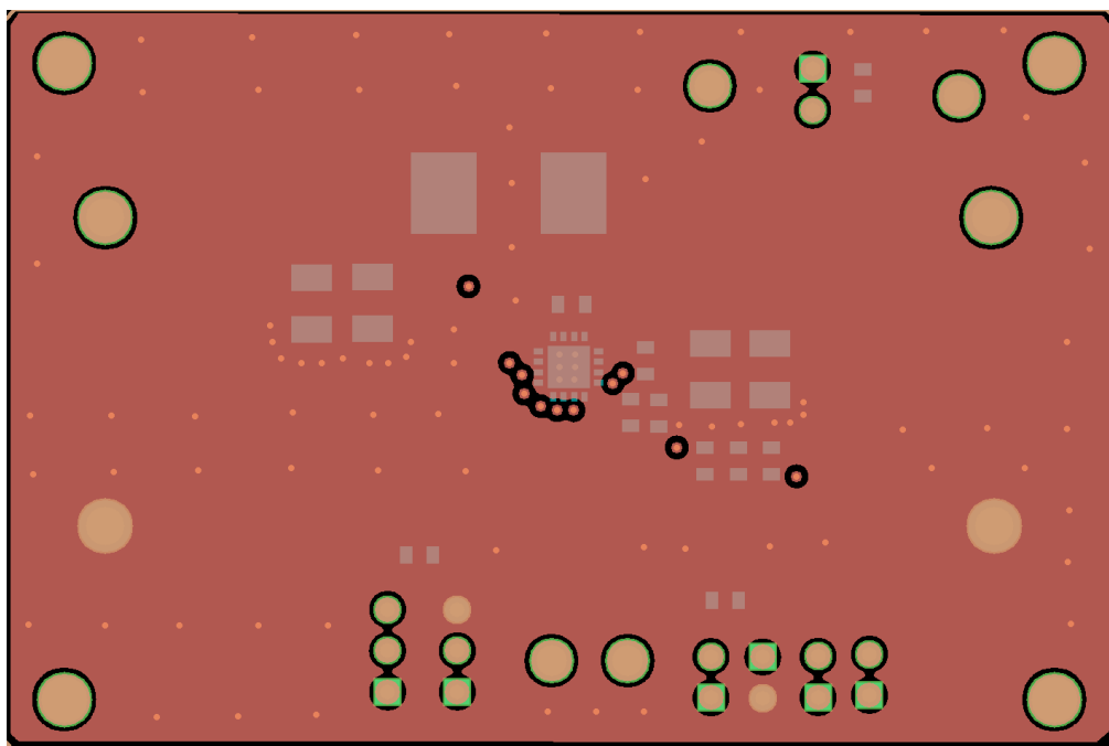
Figure 5. AP66200FVBW-EVM – Layer 2
