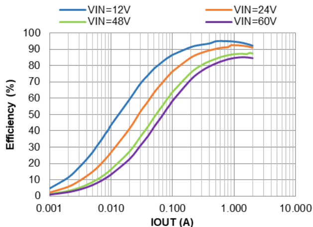
Figure 9. PWM Efficiency vs. IOUT, VOUT=5V, L=10μH
