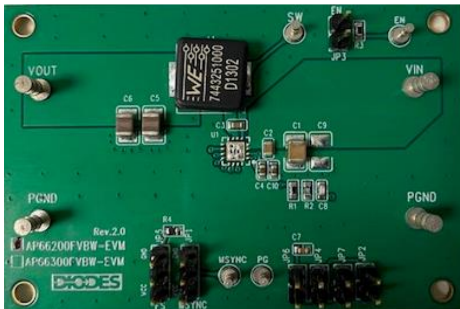
Figure 2. AP66200FVBW-EVM
