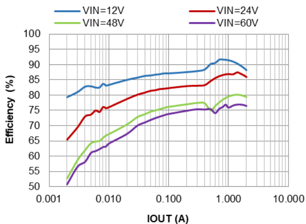
Figure 10. PFM Efficiency vs. IOUT, VOUT=3.3V, L=8.2μH
