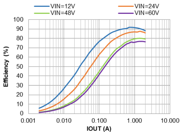
Figure 11. PWM Efficiency vs. IOUT, VOUT=3.3V, L=8.2μH
