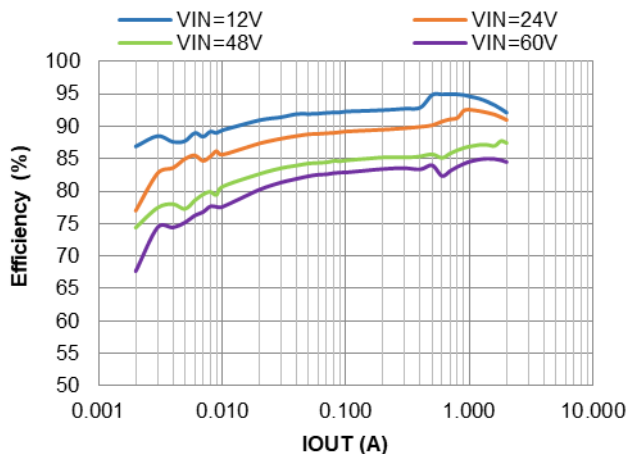
Figure 8. PFM Efficiency vs. IOUT, VOUT=5V, L=10μH
