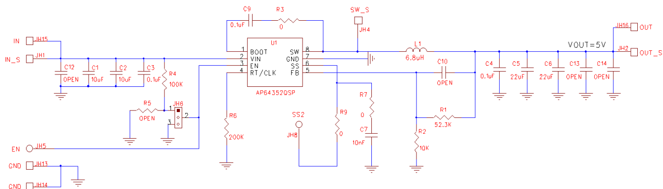
Figure 3. AP64352QSP-EVM Schematic
