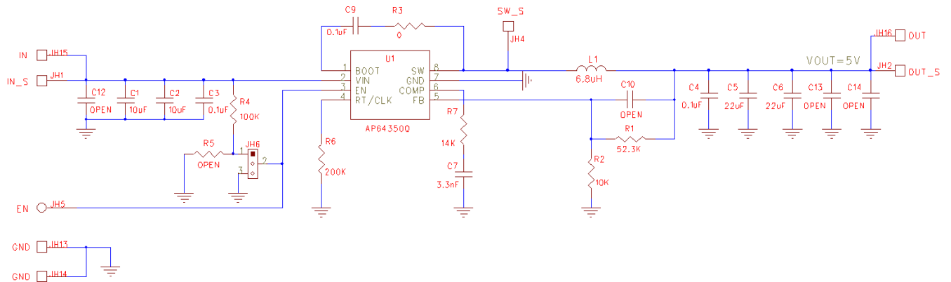
Figure 3. AP64350QSP-EVB Schematic
