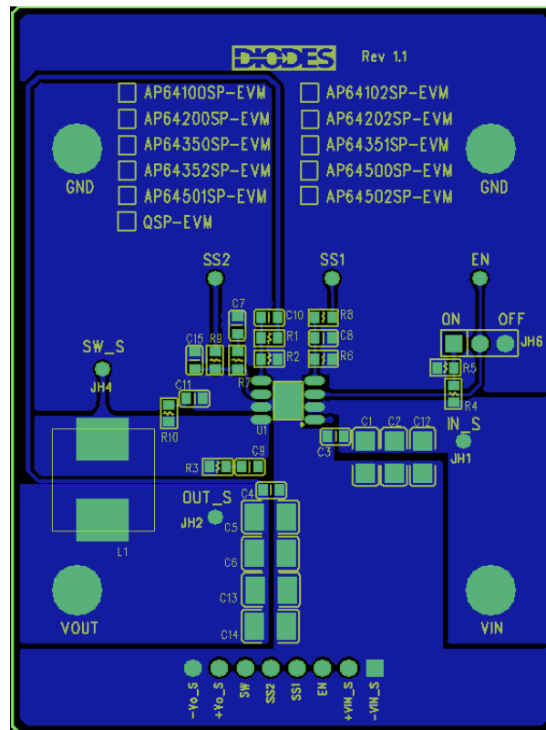
Figure 4. AP64350QSP-EVB – Top Layer
