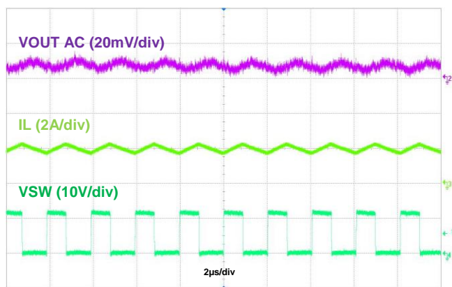
Figure 8. Output Voltage Ripple, IOU=2A
