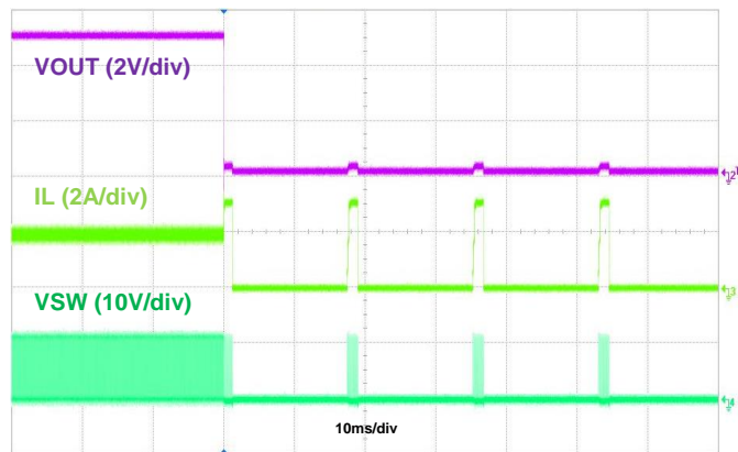
Figure 9. Output Short Protection, IOU=2A
