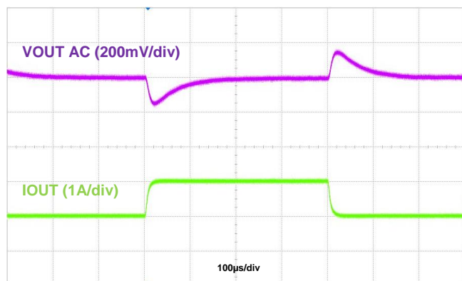
Figure 7. Load Transient 1A to 2A
