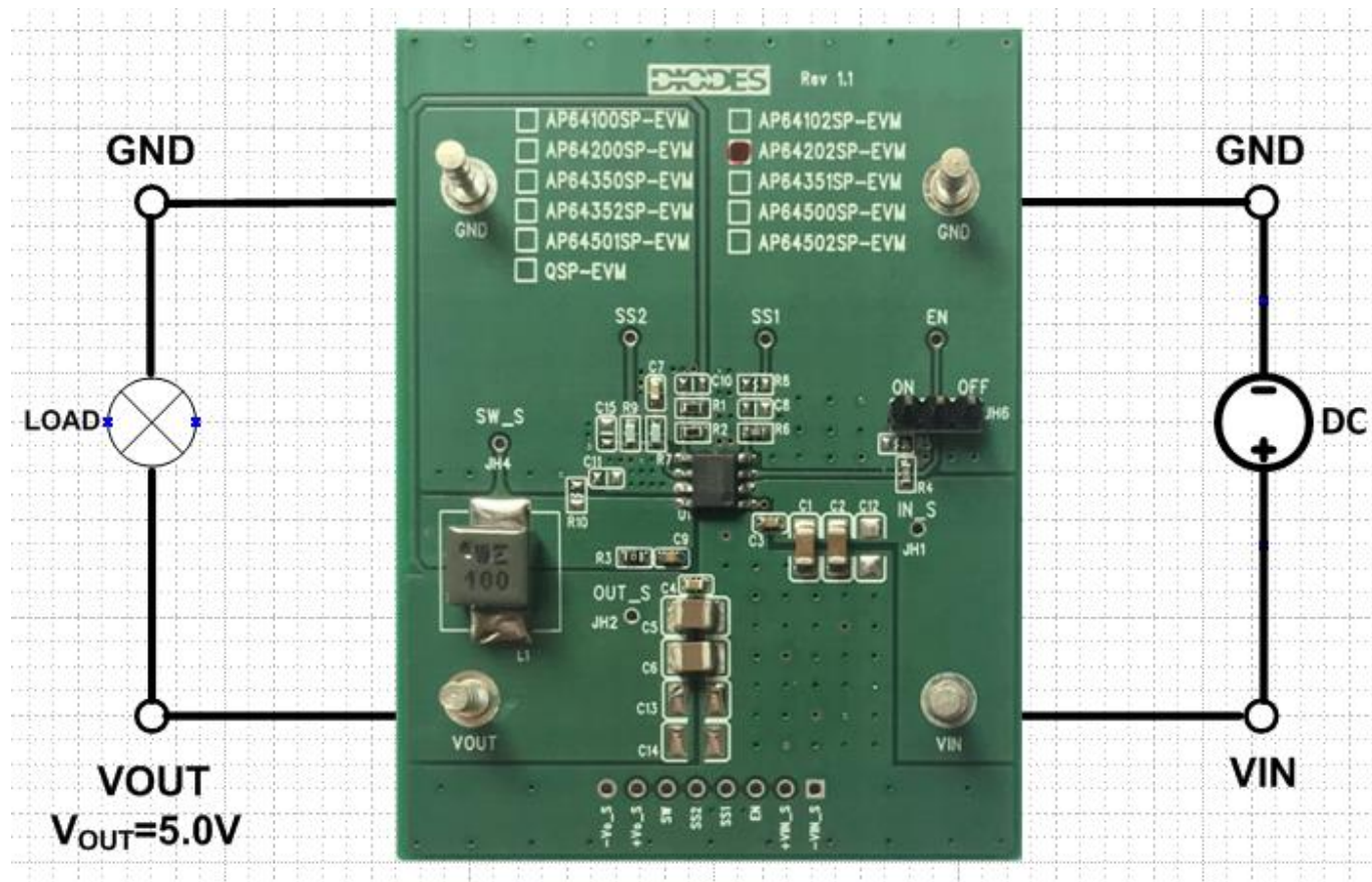
Figure 2. AP64202SP-EVM
