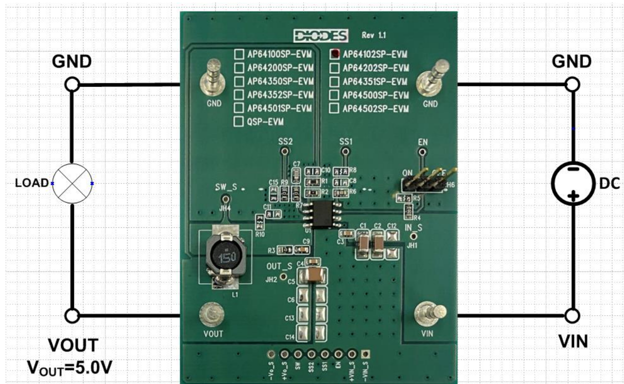
Figure 1. AP64102SP-EVM
