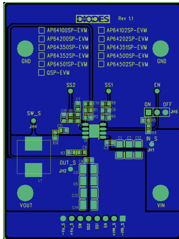
Figure 3. AP64102SP-EVB – Top Layer
