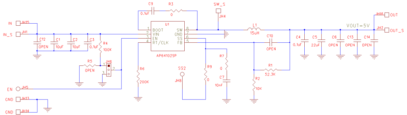
Figure 2. AP64102SP-EVB Schematic
