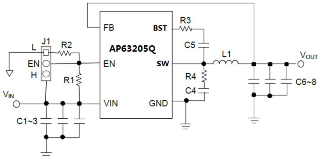
Figure 3. AP63205QWU-EVM Schematic
