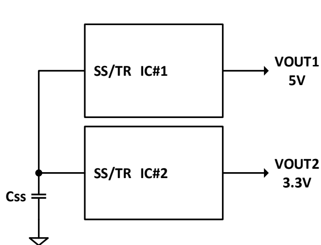
Figure 47. Ratiometric Tracking Configuration
