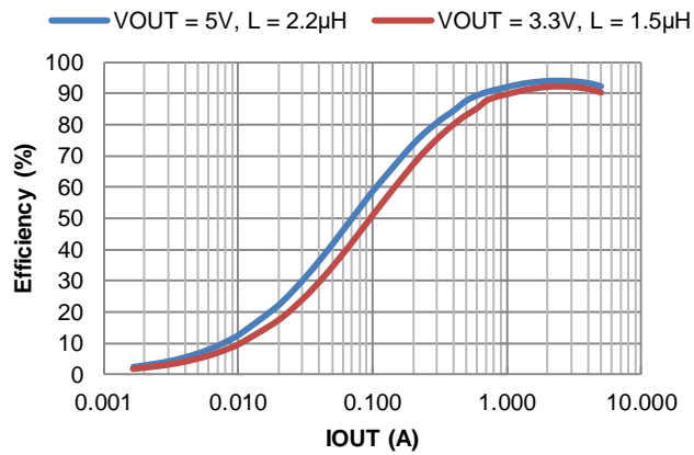
Figure 36. Efficiency vs. Output Current
