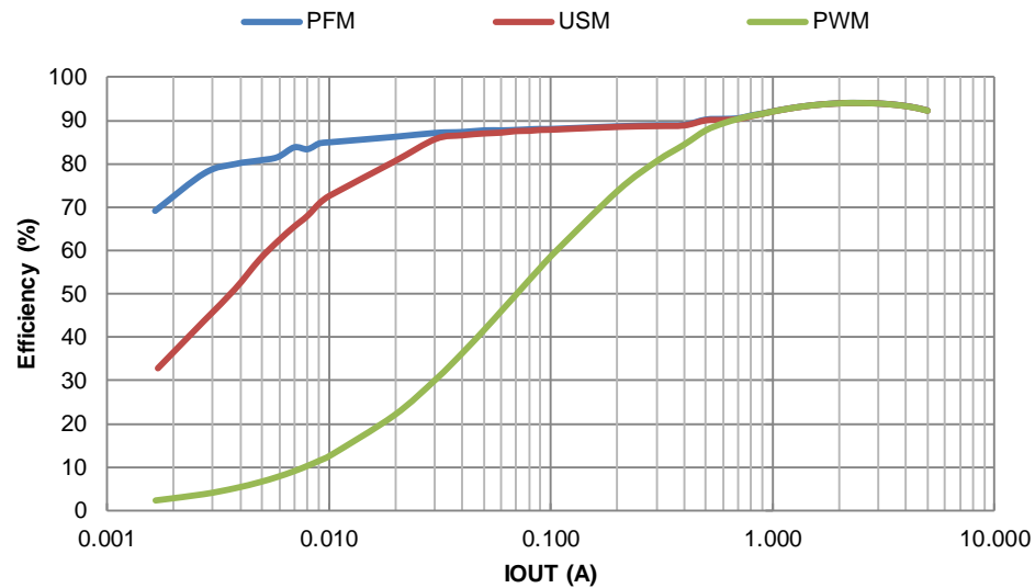
Figure 2. Efficiency vs. Output Current, VIN = 12V, VOUT = 5V, L = 2.2μH, fsw = 800kHz
