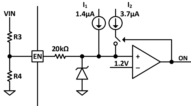
Figure 53. Programming UVLO
