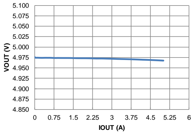
Figure 38. Load Regulation
