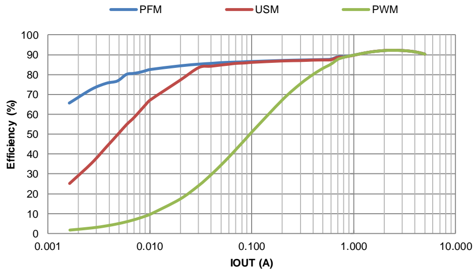
Figure 3. Efficiency vs. Output Current, VIN = 12V, VOUT = 3.3V, L = 1.5μH, fsw = 800kHz
