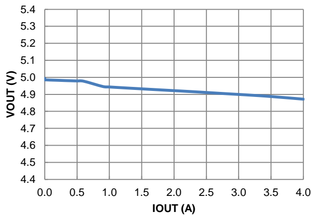
Figure 15. Load Regulation
