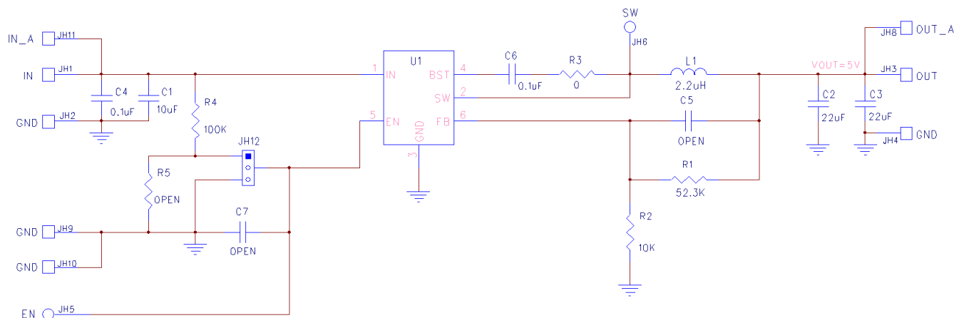
Figure 3. AP62250Z6-EVM Schematic
