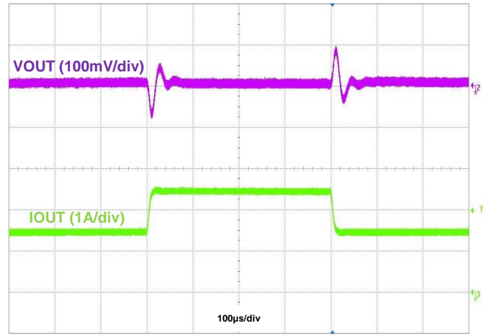
Figure 18. Load Transient, I_{OUT} = 1.5\text{A} to 2.5\text{A} to 1.5\text{A}
