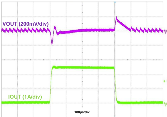
Figure 19. Load Transient, I_{OUT} = 50\text{mA} to 2.5\text{A} to 50\text{mA}
