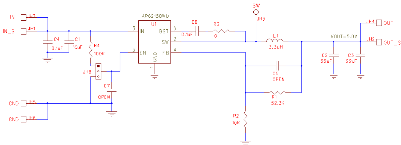
Figure 3. AP62150WU-EVM Schematic
