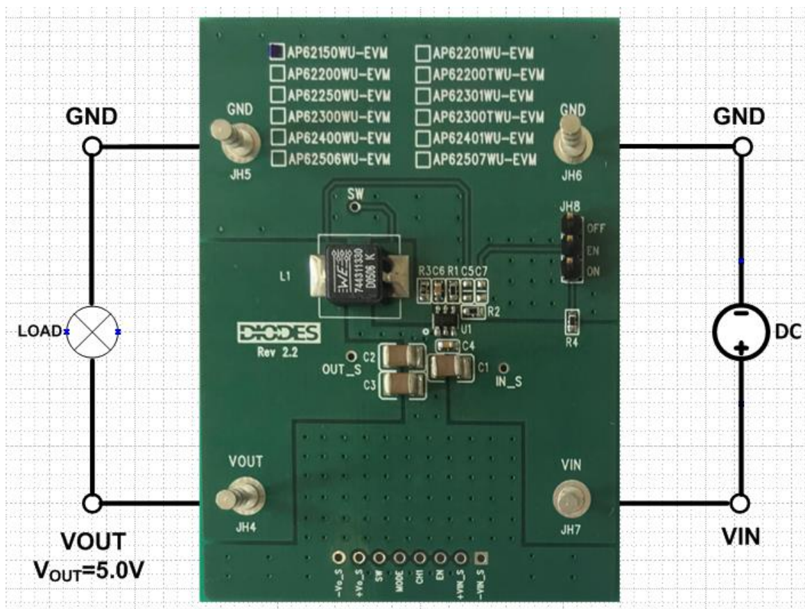
Figure 2. AP62150WU-EVM
