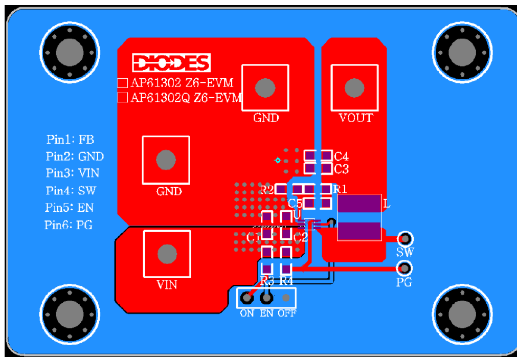
Figure 3. AP61302QZ6 - EVM - Top Layer
