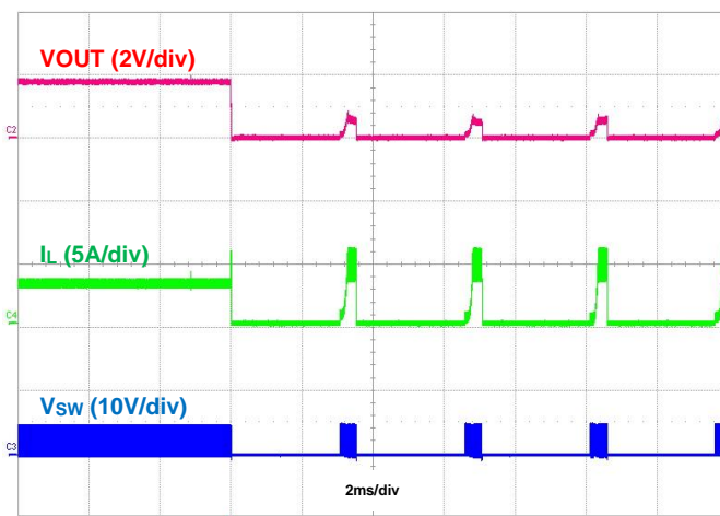
Figure 35. Output Short Protection, IOU = 3A
