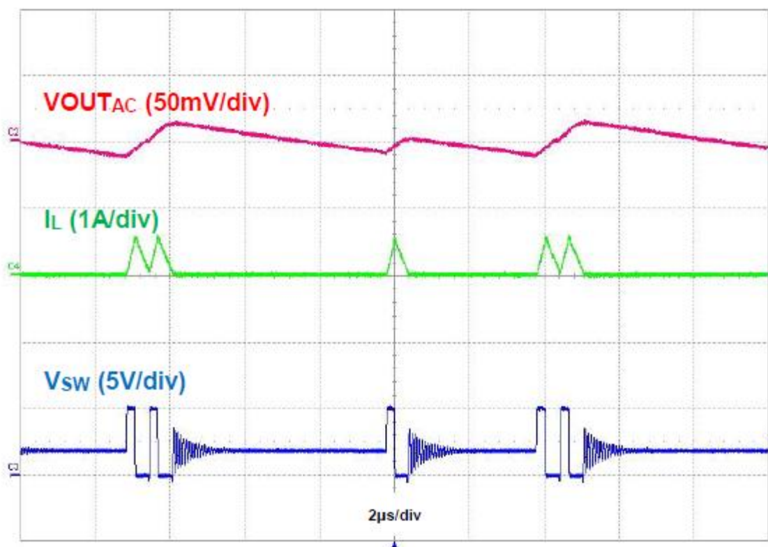
Figure 8. Output Voltage Ripple, IOUT = 50mA
