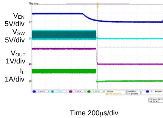
Figure 17. Enable Turn Off ( I_{OUT}=1.2A )
