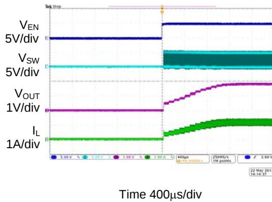
Figure 16. Enable Turn On ( I_{OUT}=1.2A )
