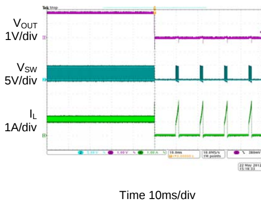
Figure 18. Short Circuit Protection ( I_{OUT}=1.2A )
