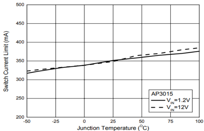
Fig 4. Switch Current Limit vs Junction Temp
