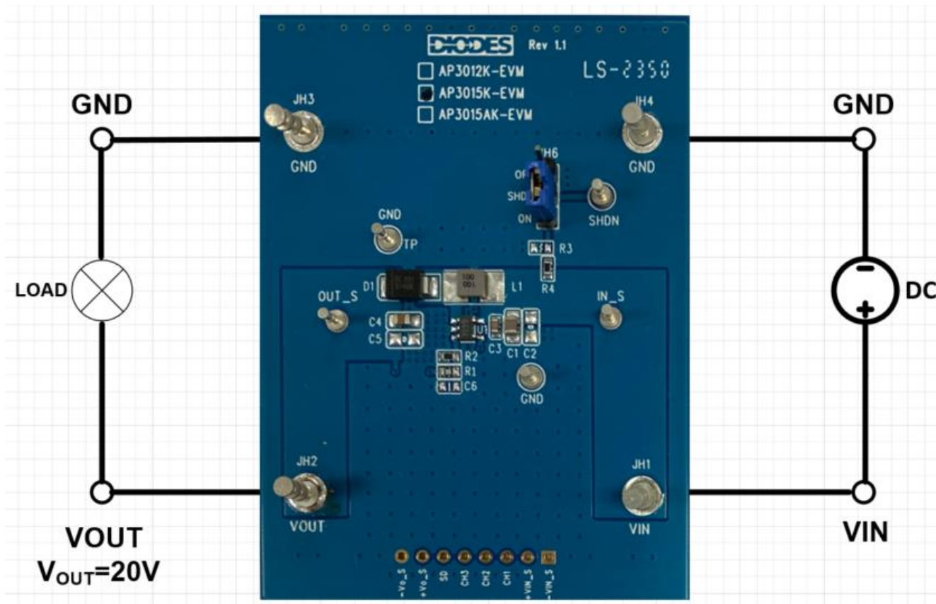
Figure 1. AP3015K-EVM
