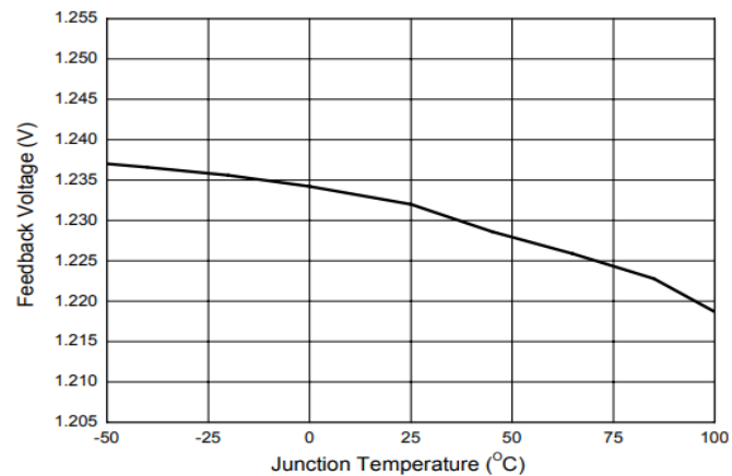
Fig 6. Feedback Voltage vs Junction Temp
