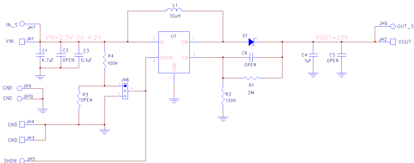
Figure 2. AP3015K-EVM Schematic
