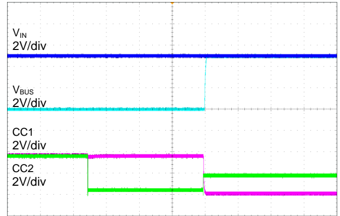
IN1 = IN2 = AUX = EN = CHG = CHG\_HI = 5\text{V} , CC1 = open , CC2 = open \rightarrow Rd
