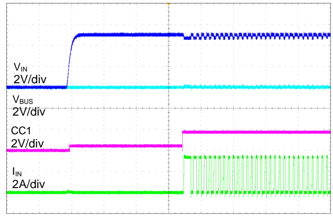
IN1 = IN2 = AUX = EN = CHG = CHG\_HI = 5\text{V} , CC1 = Rd , CC2 = open , OUT = shorted
