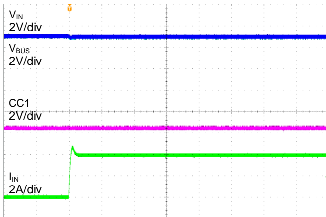
IN1 = IN2 = AUX = EN = 5\text{V} ; CHG = CHG\_HI = 0\text{V} , CC1 = open , CC2 = Rd , OUT = open \rightarrow 5\Omega
