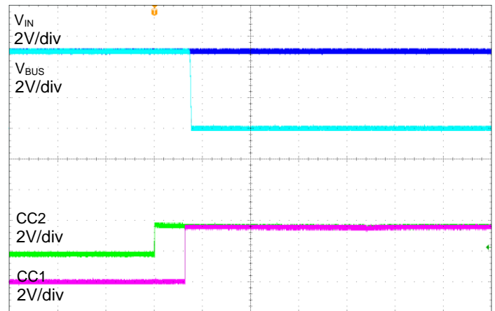
IN1 = IN2 = AUX = EN = CHG = CHG\_HI = 5\text{V} , CC1 = open , CC2 = Rd \rightarrow open
