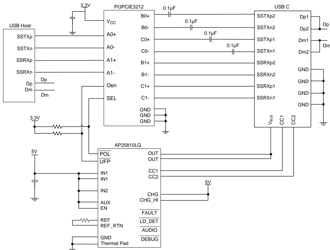
Figure 22. Example Implementation
