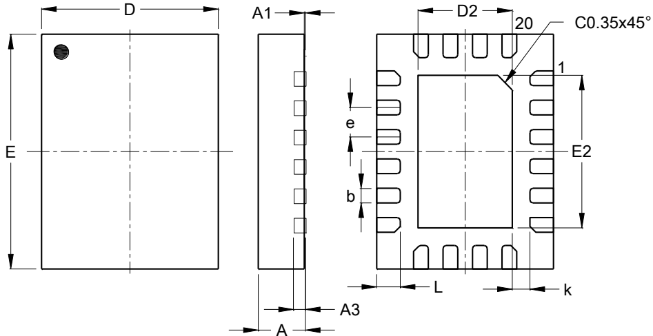
W-QFN3040-20 (Type A1)
