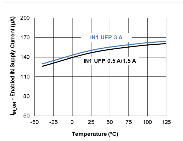
Figure 8. IN1 Current with UFP vs. Temperature
