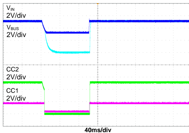
Figure 17. Brown-Out Test
