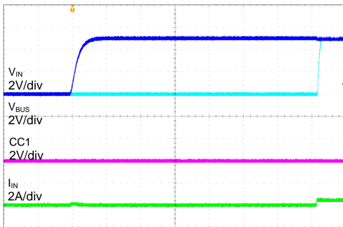
IN1 = IN2 = AUX = EN = CHG = CHG\_HI = 5\text{V} , CC1 = short , CC2 = Rd
