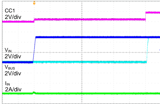
Basic start-up: IN1 = IN2 = AUX = EN = CHG = CHG\_HI = 5\text{V} , CC1 = Rd , CC2 = open
