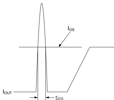
Figure 1. Output Short-Circuit Timing Diagram
