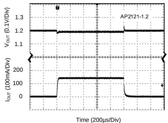
Load Transient (Conditions: V_{IN} = 2.2V , C_{IN} = 1\mu F , C_{OUT} = 1\mu F )
