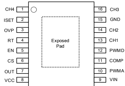
TSSOP-16EP (Type DX)
