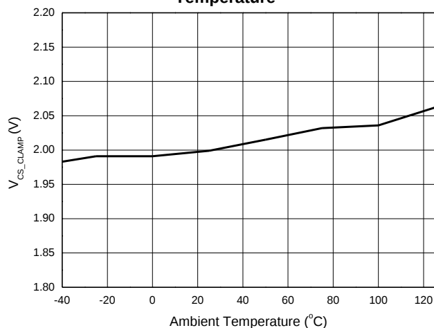
CS Clamp Reference Voltage vs. Ambient Temperature
