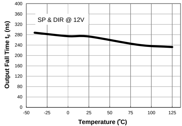
Output Fall Time t_F vs. Temperature
