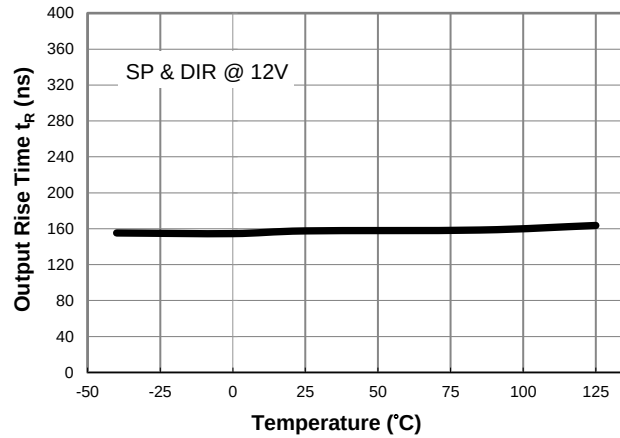
Output Rise Time t_R vs. Temperature
