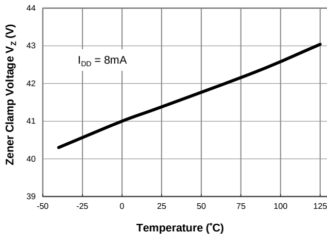
Zener Clamp Voltage V_Z vs. Temperature
