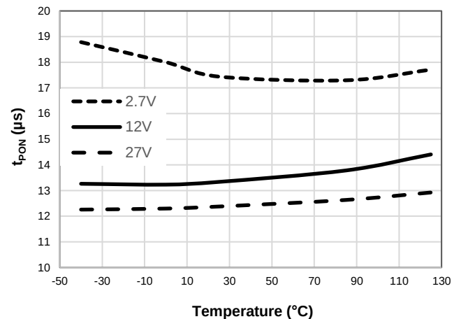
t_{PON} vs. Temperature
