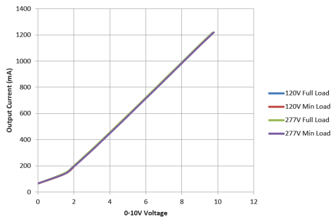
LC50-1200D-UNV-T Dimming Curve (0-10V)
