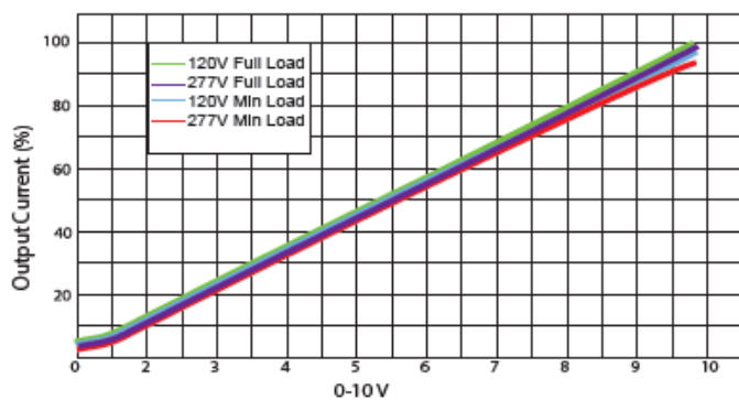
Dimming Curve - 0-10V Dimming
