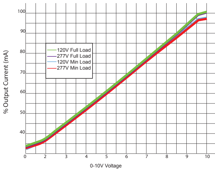
Dimming Curve
