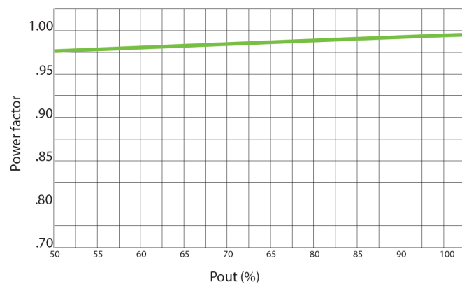
Power Factor vs. Output Power - 0-10 Dimming
