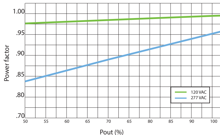
Power Factor vs. Output Power - Non-Dimming
