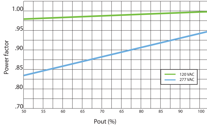
Power Factor vs. Output Power - 0-10 Dimming
