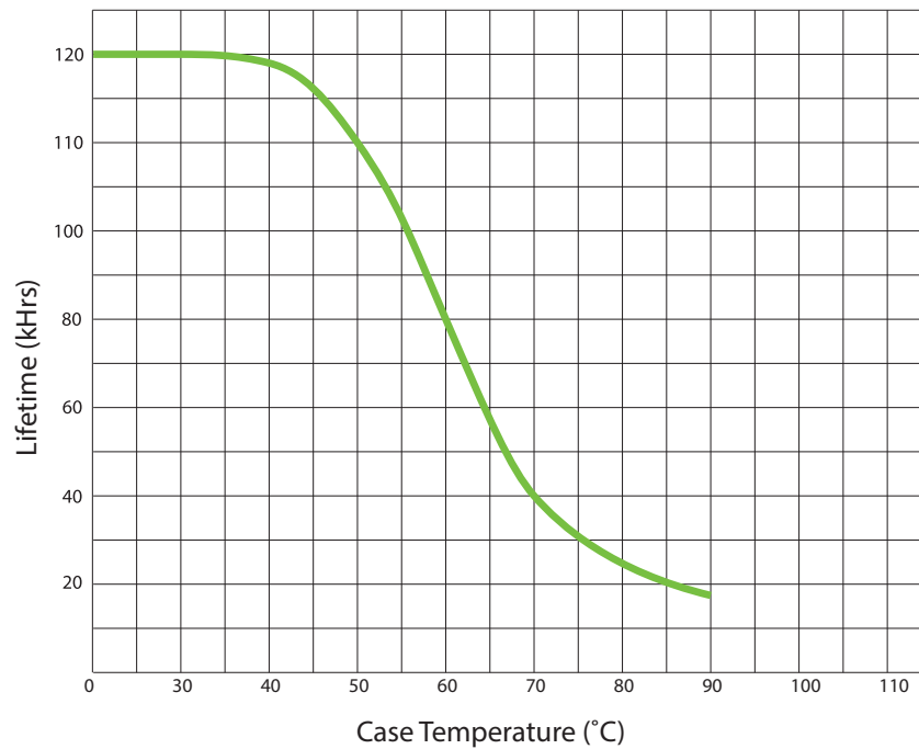
Lifetime vs. Case Temperature
