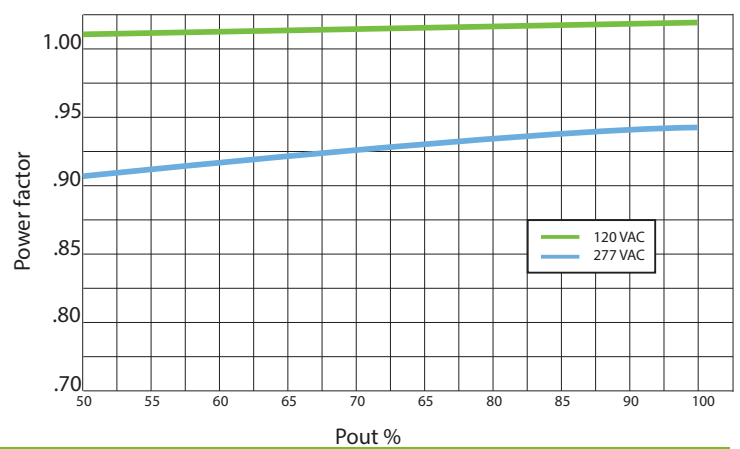
Power Factor vs. Output Power - 0-10V Dimming
