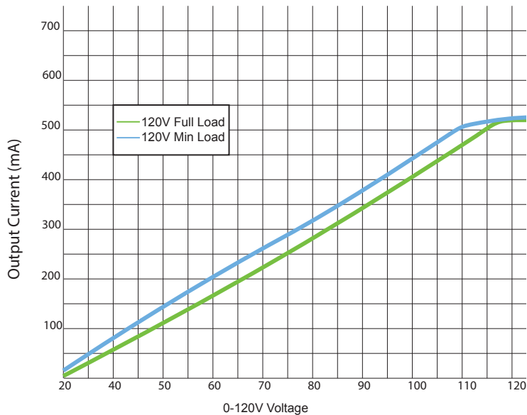
Dimming Curve
