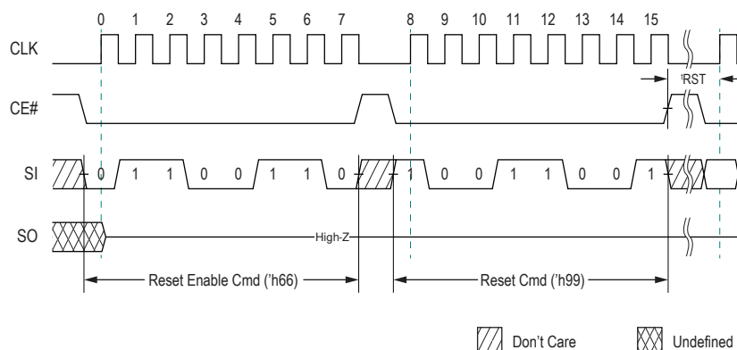
Figure 23: SPI Reset
