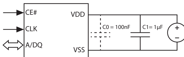
Figure 27: Decoupling Capacitor
