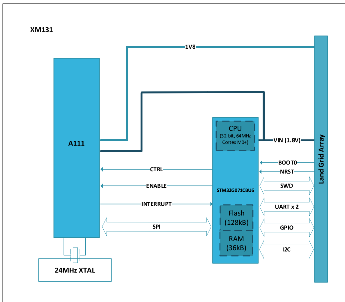
Figure 2. XM131 block diagram.
