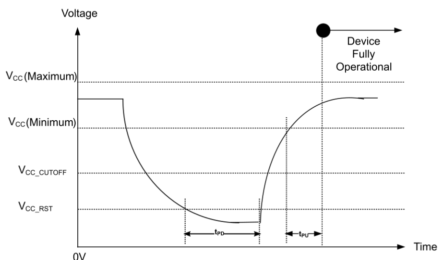
Figure 10: Power-Down Behavior
