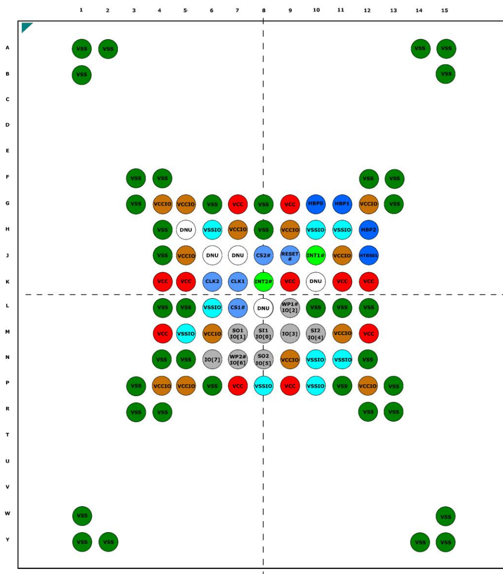
Figure 5: 96-ball FBGA
