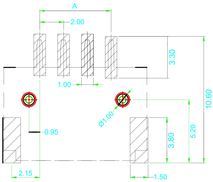
P. C. B LAYOUT
