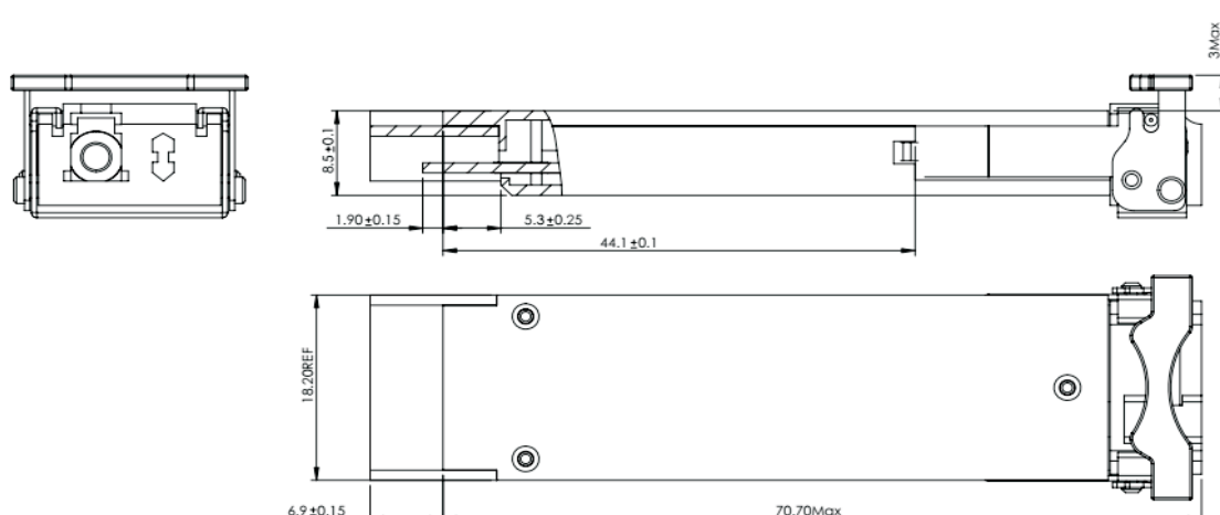
APXBxxB30CDL70(dimensions are in mm)
