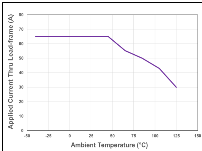
Figure 28. CT432 Current De-rating Curve for 65 A DC
