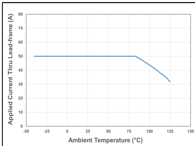
Figure 22. CT432 Current De-rating Curve for 50 A DC
