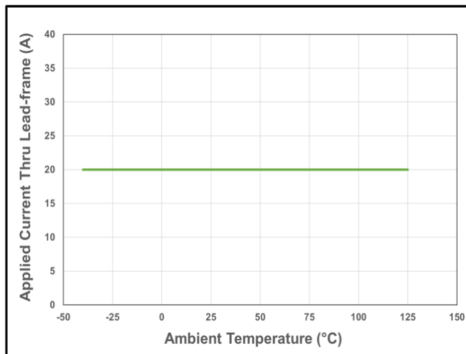
Figure 10. CT432 Current De-rating Curve for 20 A DC
