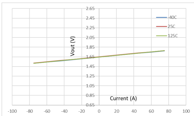
FIGURE 3. EXCELLENT LINEARITY AND TEMPERATURE PERFORMANCE FOR CTD453
