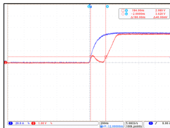
Figure 7: CT432 Propagation Delay; I_P = 50 \text{ A}_{PK} and C_L = 100 \text{ pF} (Blue = I_{CCC} , Red = V_{OUT} )
