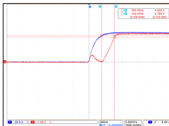
Figure 5: CT432 Response Time; I_P = 50 \text{ A}_{PK} and C_L = 100 \text{ pF} (Blue = I_{CCC} , Red = V_{OUT} )
