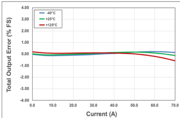
Figure 32: Total Output Error vs. Current vs. Temperature
