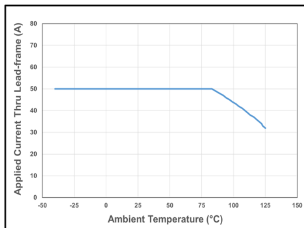
Figure 22: CT432 Current Derating Curve for 50 A DC
