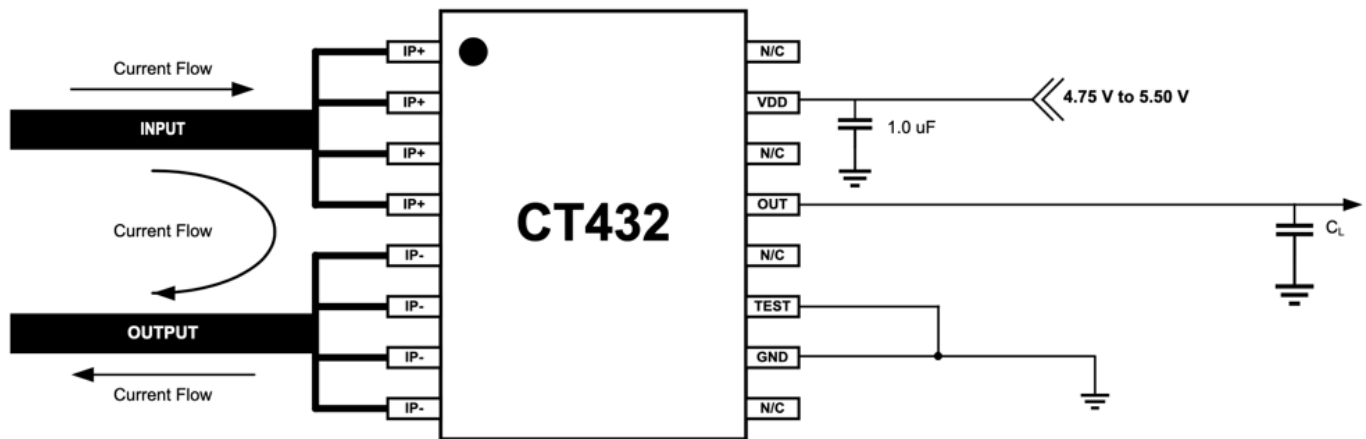
Figure 39: CT432 Application Block Diagram
