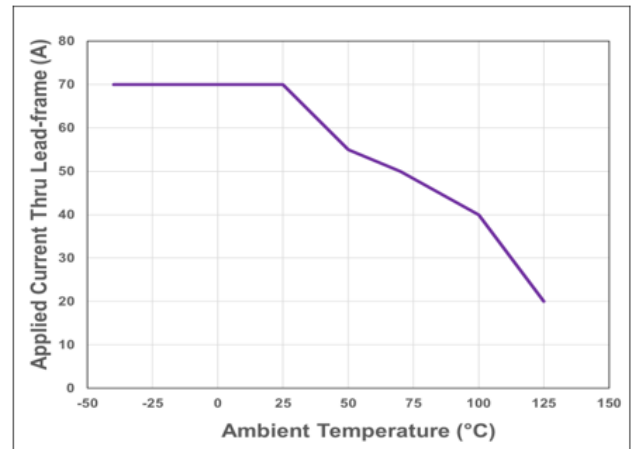
Figure 33: CT432 Current Derating Curve for 70 A RMS
