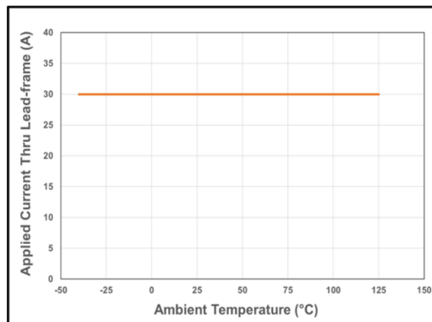
Figure 16: CT432 Current Derating Curve for 30 A DC
