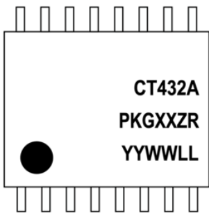
Figure 44: CT432 Device Marking for 16-lead Package
