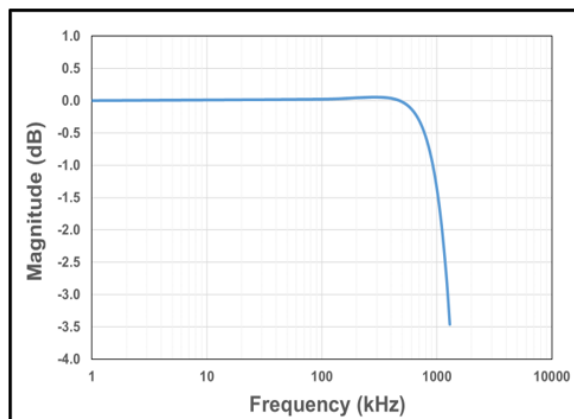
Figure 4: CT432 Bandwidth
