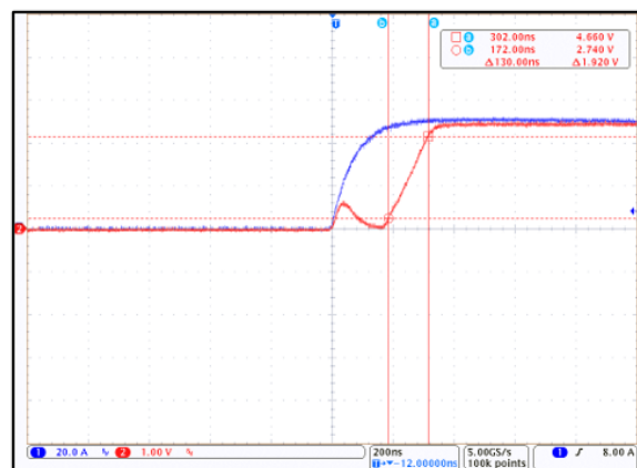
Figure 6: CT432 Rise Time; I_P = 50 \text{ A}_{PK} and C_L = 100 \text{ pF} (Blue = I_{CCC} , Red = V_{OUT} )
