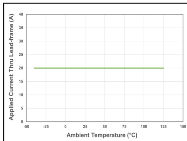
Figure 10: CT432 Current Derating Curve for 20 A DC
