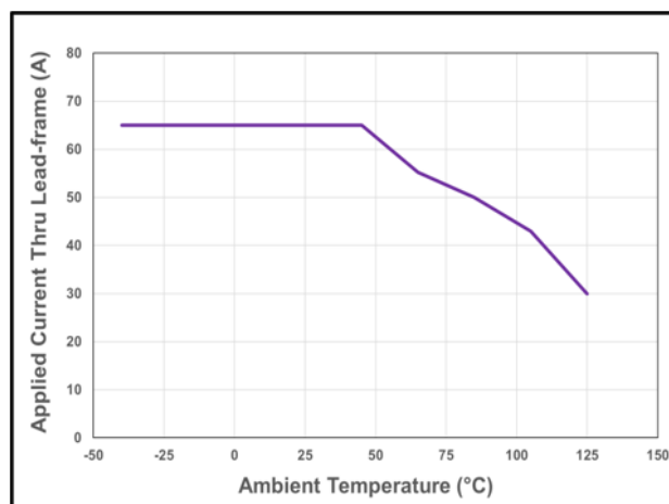
Figure 28: CT432 Current Derating Curve for 65 A DC
