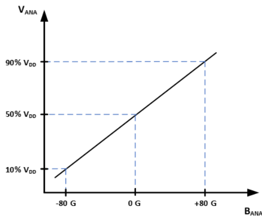
Figure 27: Linear Output Voltage Range vs. Measured Magnetic Field for S = 5 \text{ mV/V/G} .
