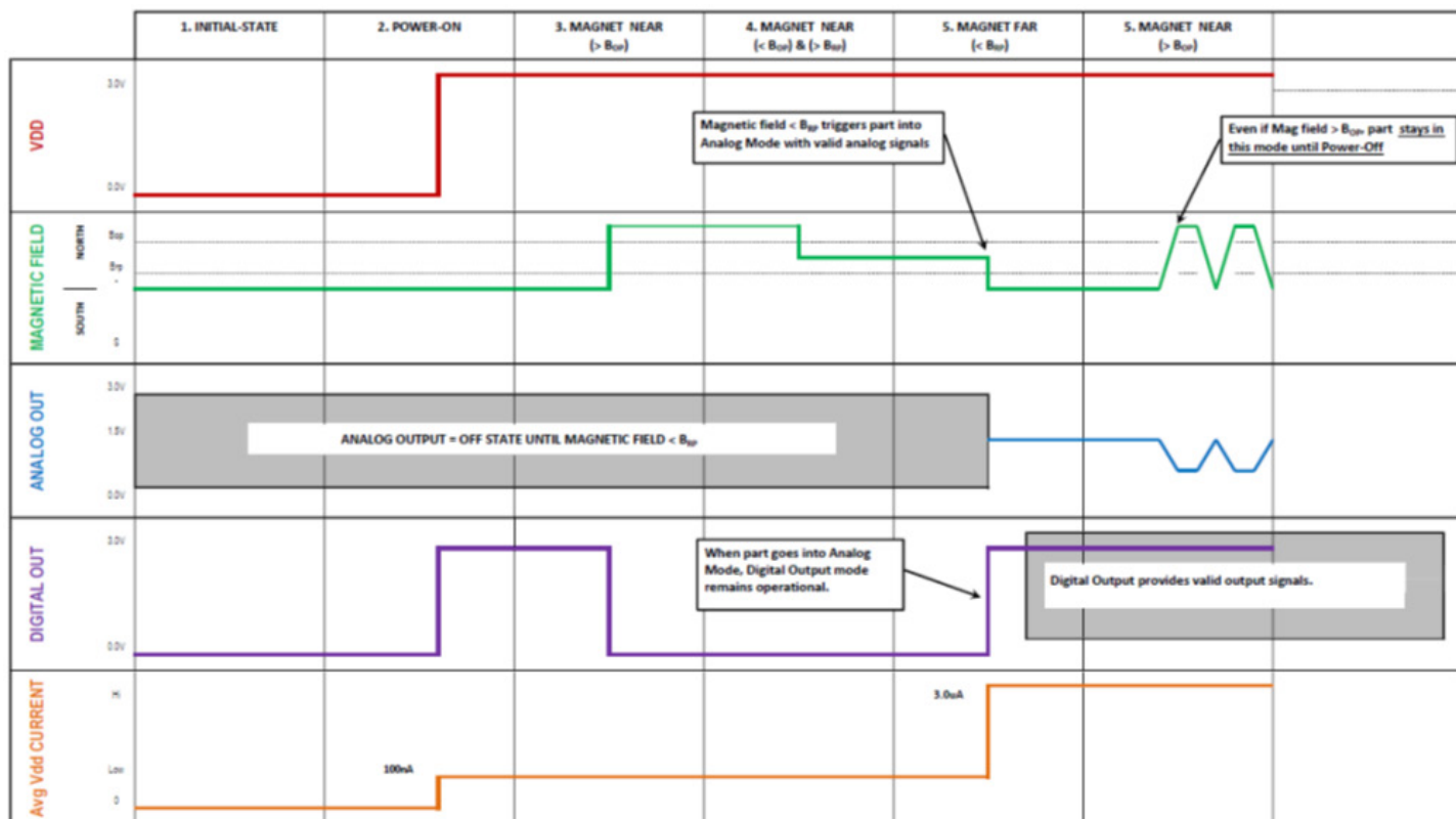
Figure 30: Dual Analog and Digital Mode Operating Conditions of the CT8152.
