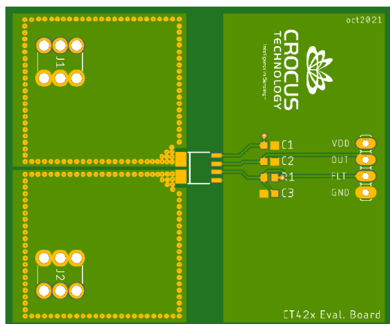
Figure 43: Recommended PCB Layout (Top Layer) for the 20 A to 65 A variants of the CT417
