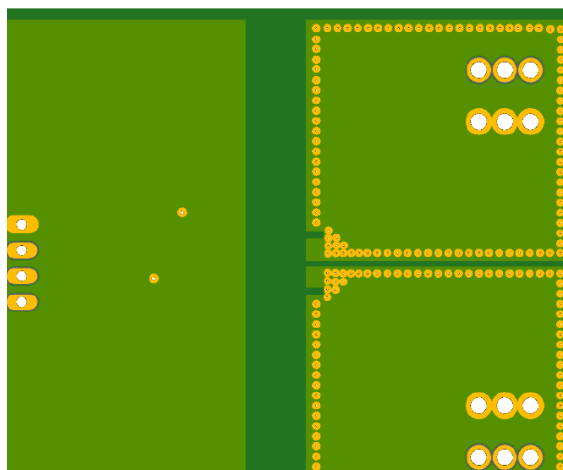
Figure 44: Recommended PCB Layout (Bottom Layer) for the 20 A to 65 A variants of the CT417
