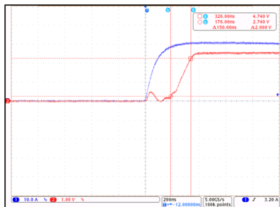
Figure 9: CT415 Rise Time; I_P = 30 \text{ A}_{PK} and C_L = 100 \text{ pF} (Blue = I_{CCC} , Red = V_{OUT} )
