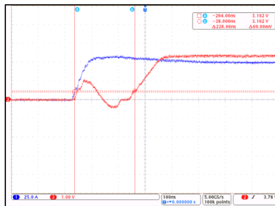
Figure 10: CT415 Propagation Delay; I_P = 30 \text{ A}_{PK} and C_L = 100 \text{ pF} (Blue = I_{CCC} , Red = V_{OUT} )
