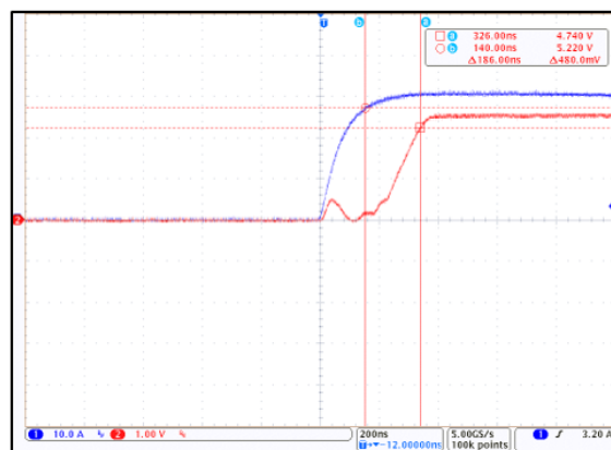
Figure 8: CT415 Response Time; I_P = 30 \text{ A}_{PK} and C_L = 100 \text{ pF} (Blue = I_{CCC} , Red = V_{OUT} )
