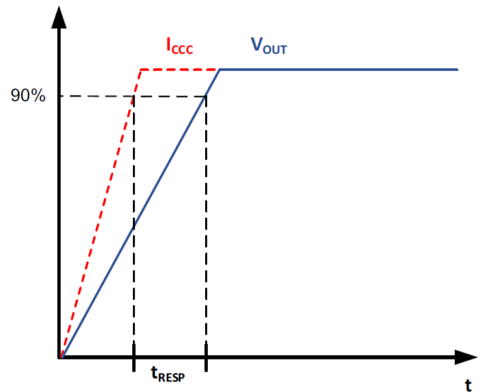
Figure 38: CT415 Response Time Curve
