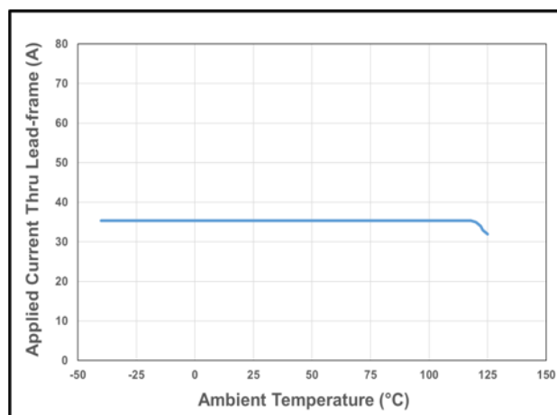
Figure 39: CT430 Current Derating Curve for 50 A_{PK} (35.4 A_{DC} )
