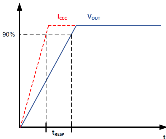
Figure 40: CT428 Response Time Curve
