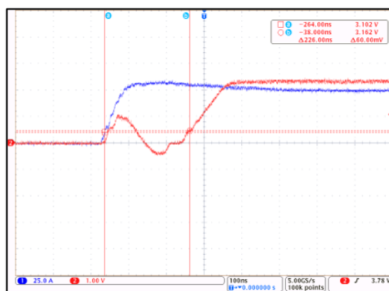
Figure 9: CT428 Propagation Delay; I_P = 30 \text{ A}_{PK} and C_L = 100 \text{ pF} (Blue = I_{CCC} , Red = V_{OUT} )
