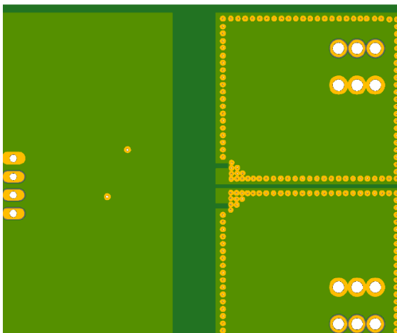
Figure 44: Recommended PCB Layout (Bottom Layer) for the 20 A to 65 A variants of the CT428
