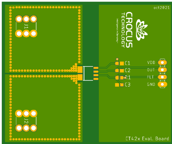
Figure 43: Recommended PCB Layout (Top Layer) for the 20 A to 65 A variants of the CT428
