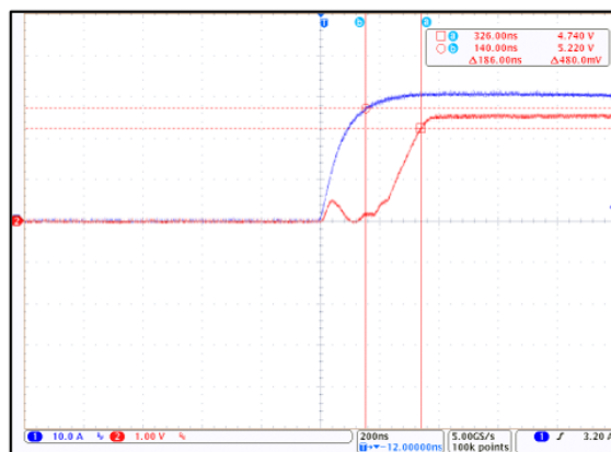
Figure 7: CT428 Response Time; I_P = 30 \text{ A}_{PK} and C_L = 100 \text{ pF} (Blue = I_{CCC} , Red = V_{OUT} )
