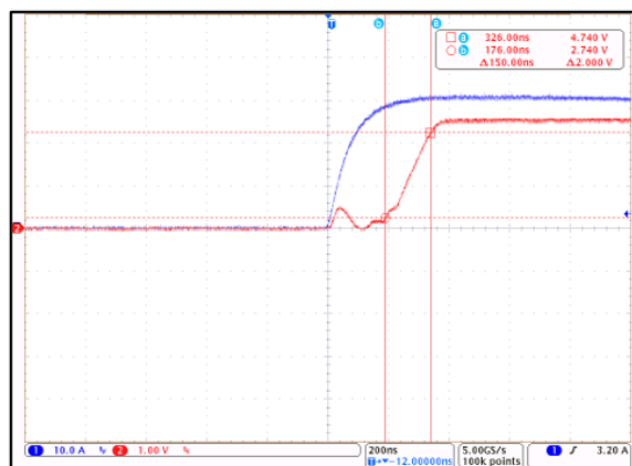
Figure 8: CT428 Rise Time; I_P = 30 \text{ A}_{PK} and C_L = 100 \text{ pF} (Blue = I_{CCC} , Red = V_{OUT} )
