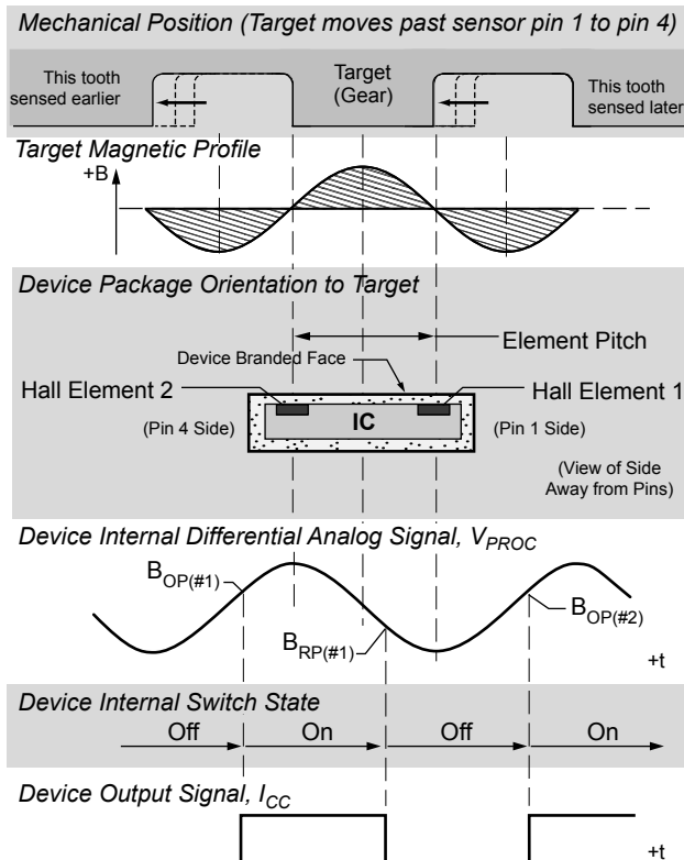
Figure 2. The magnetic profile reflects the geometry of the target, allowing the ATS685 to present an accurate digital output response.
