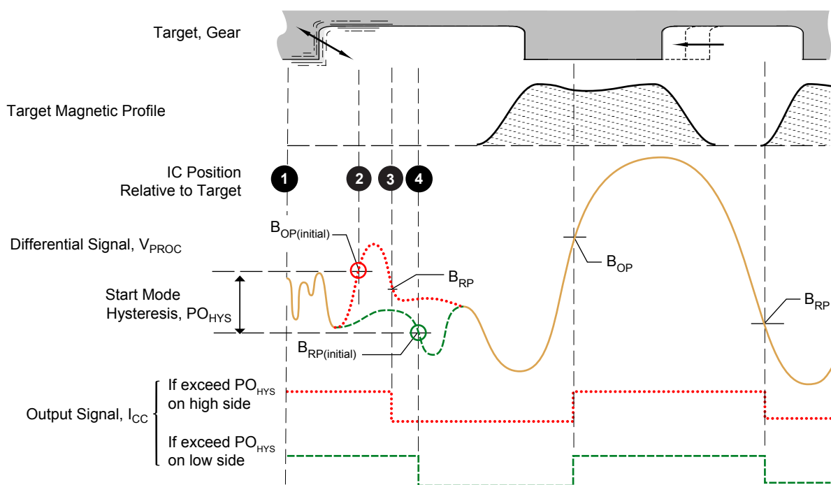
Figure 7. Operation of Start Mode Hysteresis
