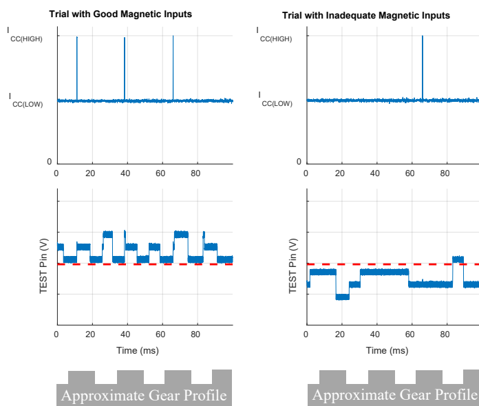
Figure 12: Example of Target Assessment signal. (a) at left, shows good signals, above threshold of goodness (b) at right, signal is below threshold
