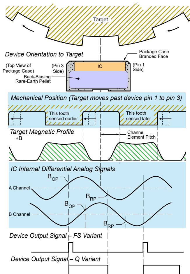
Figure 5: Magnetic Profile
