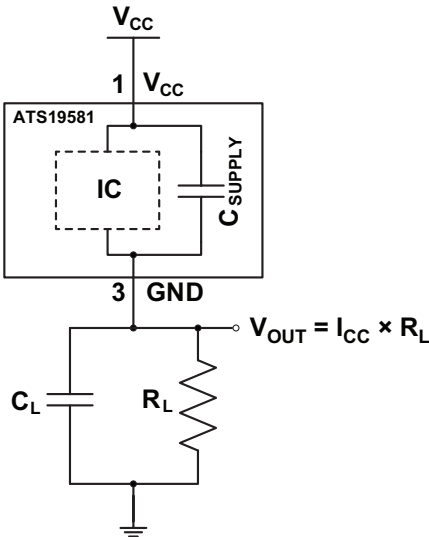
Figure 2: Typical Application Circuit
